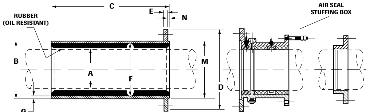
NAVAL BRASS FORWARD STERN TUBE FLANGED BEARING SCHEMATIC
